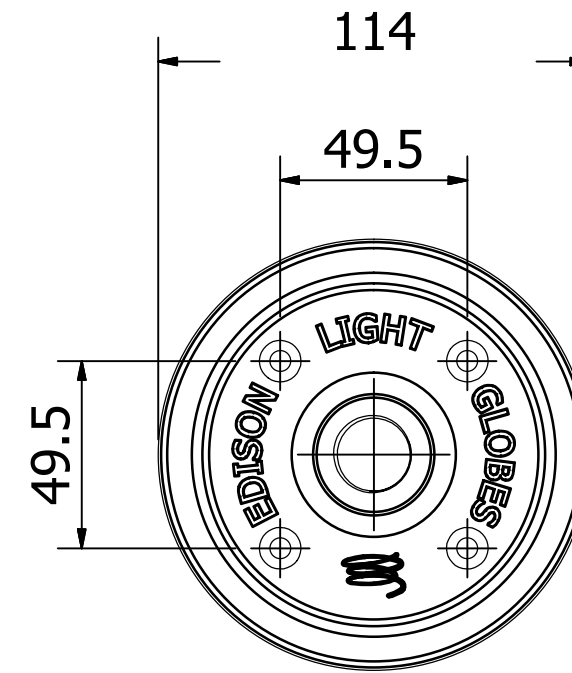
CEILING PLATE MOUNTING DETAIL
